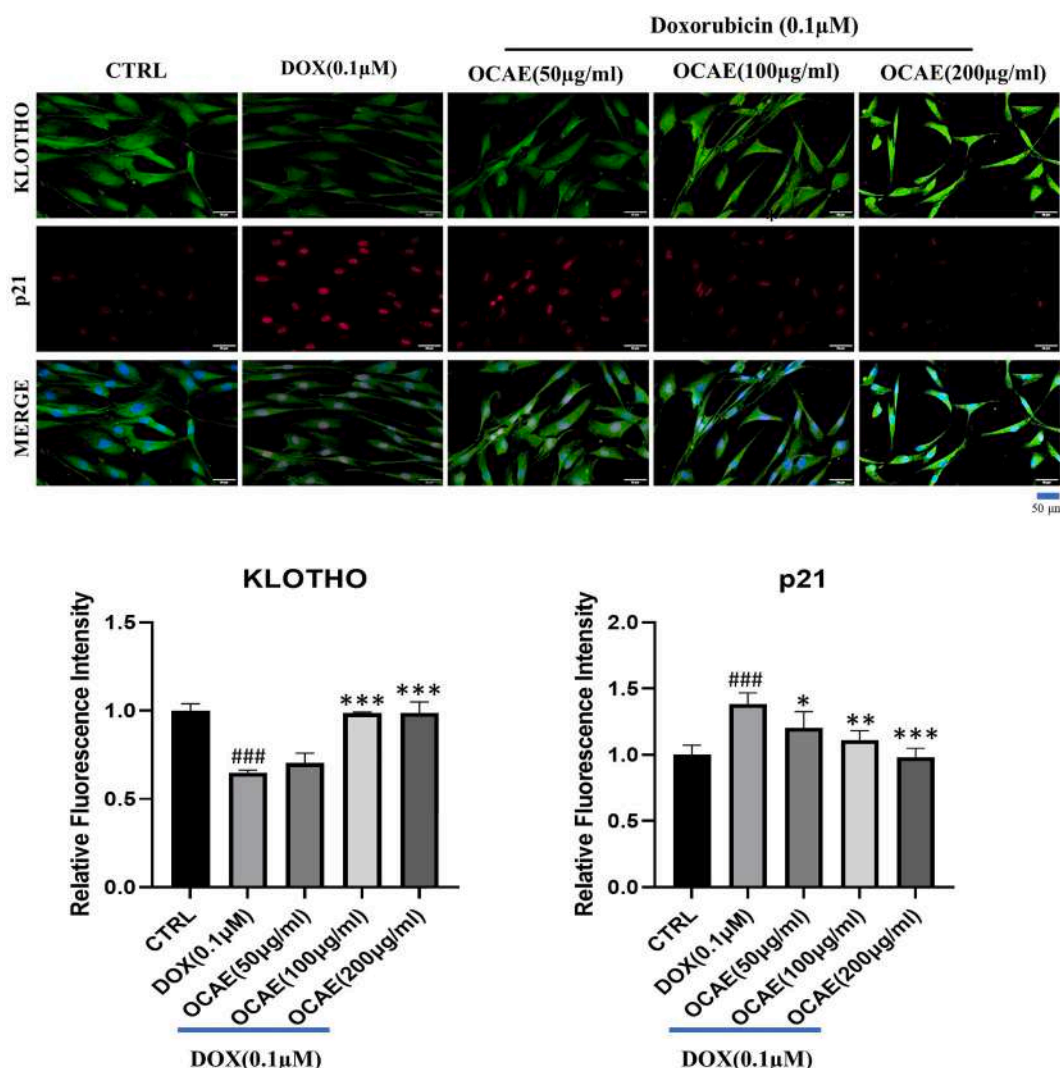
Fig. 4. The aqueous extract of O. caudata suppresses doxorubicin-induced aging in hADMSCs. After doxorubicin treatment, the hADMSCs were further treated with varying concentrations (50, 100 and 200 μg/ml) of O. caudata aqueous extract for 24 h. The cells were stained with anti-klotho (green) and anti-p21 (red) antibodies. CTRL: untreated control group. OCAE: treatment with O. caudata aqueous extract. DOX: doxorubicin. Scale bar: 50 μm. Error bars represent the standard deviation. ###p < 0.001 compared with that in the untreated control group. *p < 0.05, **p < 0.01 and ***p < 0.001 compared with that in the doxorubicin-induced aging hADMSC group. (For interpretation of the references to color in this figure legend, the reader is referred to the Web version of this article.)
